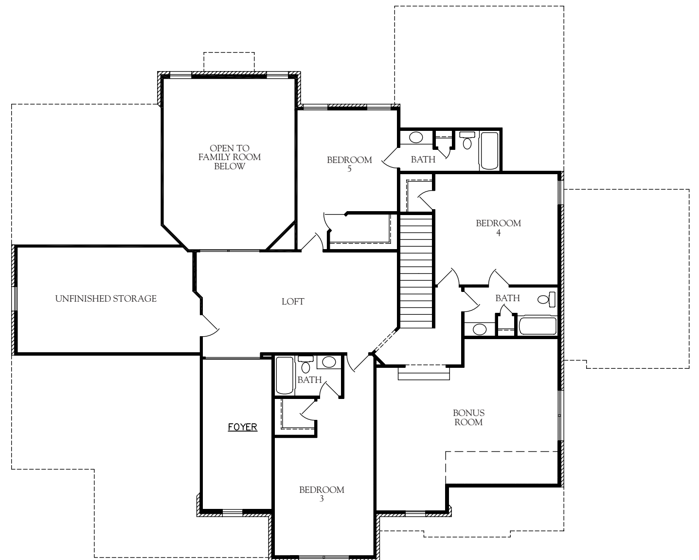
Second Floor
