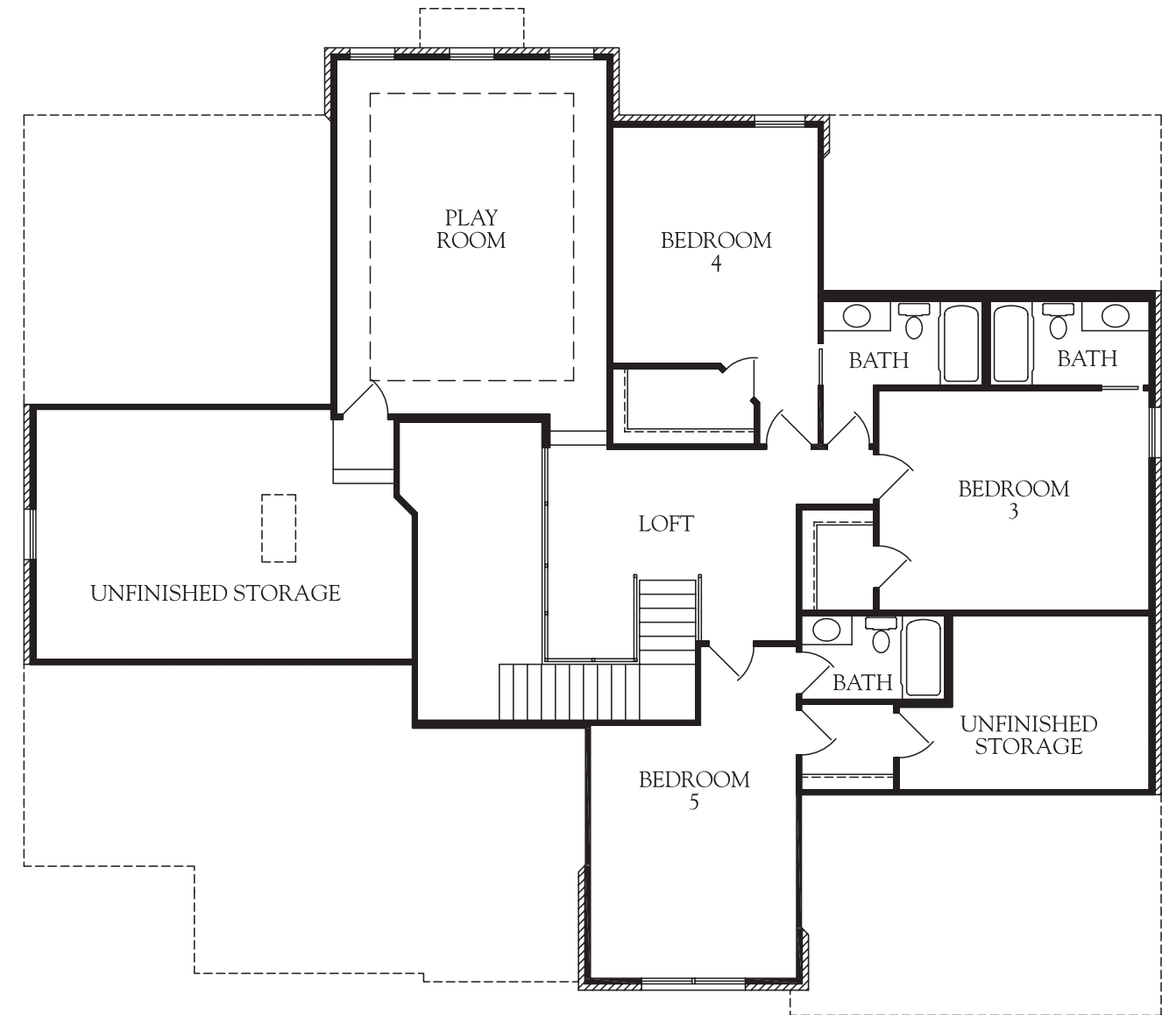
Second Floor
