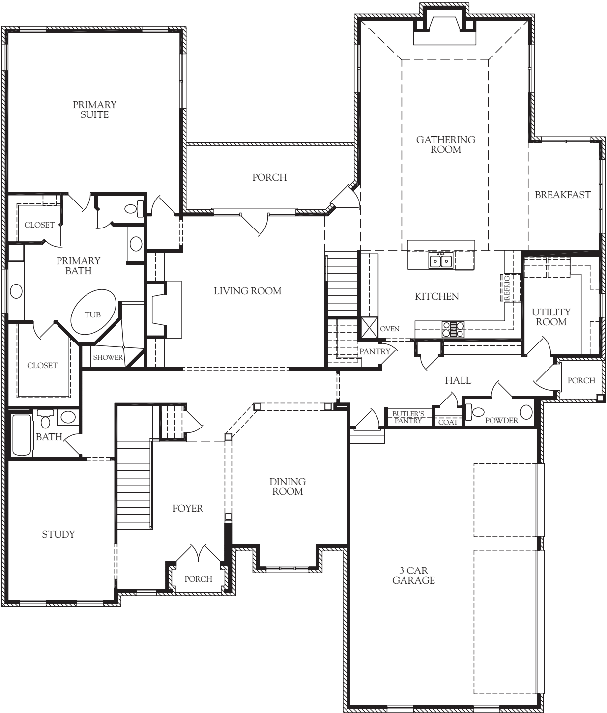
First Floor
