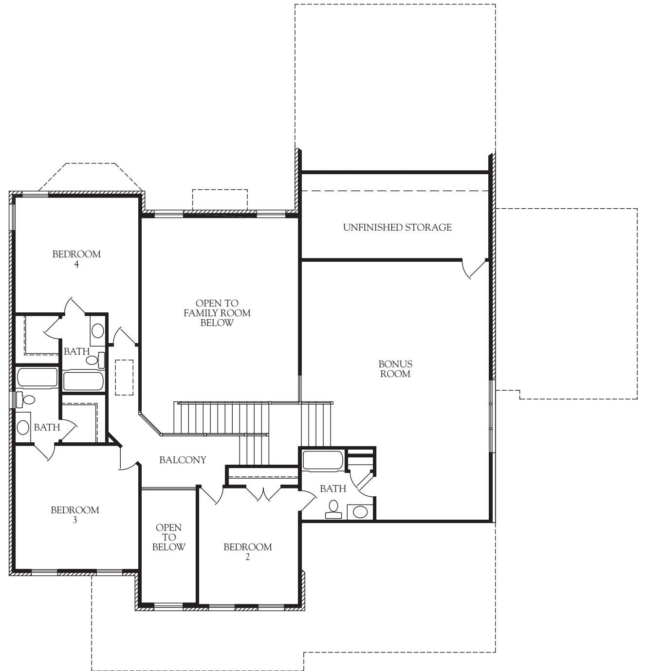
Second Floor
